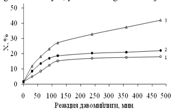
2-rasm. PAN tolasini RS1 3 bilan ta'sirlanishida nitril guruhlari o'zgarish darajasi-ning reaksiya davomiyligi bilan o'zgarishi.
